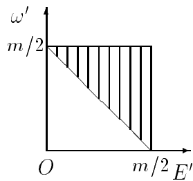
Figure 4: The shaded region is the domain of integration (99)
