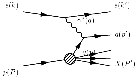
Figure 3: Parton model diagram of deep inelastic scattering.
