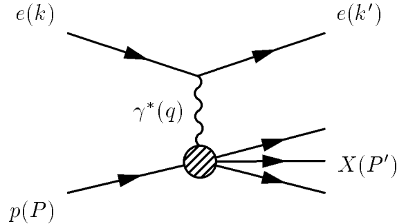
Figure 2: Generic diagram of deep inelastic scattering.
