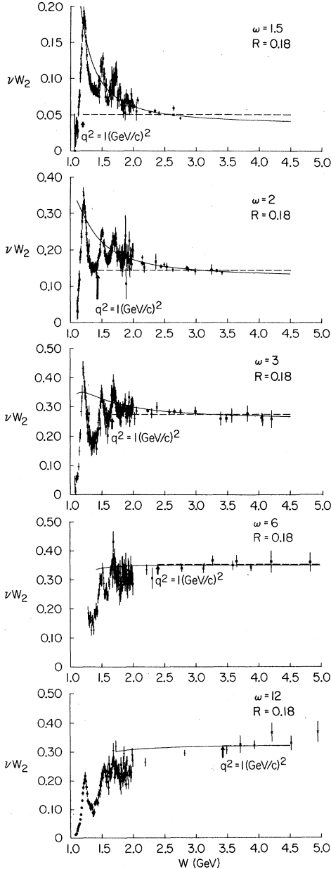
FIG. 5. Interpolated data are shown for five values of \omega = 1.5, 2, 3, 6 , and 12 . Scaling in \omega would imply a constant value of \nu W_2 as W (or q^2 ) is varied. The curved solid line represents the fit to \nu W_2 as a function of \omega' given in Eq. (6). Note that a graph with \omega constant does not have \omega' constant. The horizontal dashed line is the value of F(\omega) from Eq. (5).
