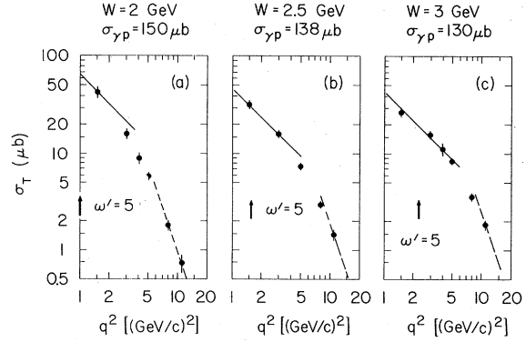
FIG. 9. The values of \sigma_T given in Table III are shown at constant W as a function of q^2 for W = 2, 2.5 , and 3.0 \text{ GeV} . The solid line indicates a 1/q^2 dependence and the dashed line represents a 1/q^6 variation with q^2 . The point \omega' = 5 is also indicated.
